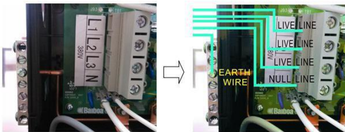
380V Diagram (L/N/E)
